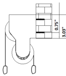
5.5" Bracket
